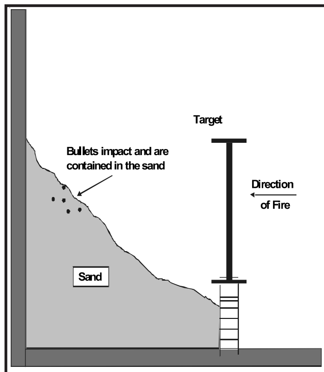
Sand Trap
